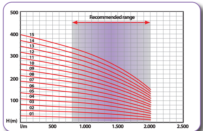
180 SEC 90 series operating curves
