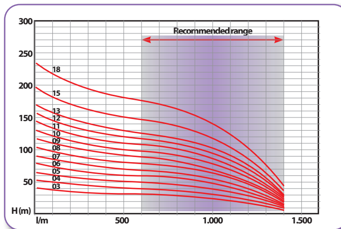
140 SEC 66 series operating curves
