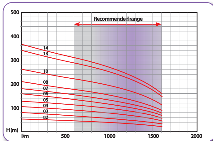
180 SEC 78 series operating curves
