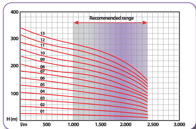
180 SEC 102 series operating curves
